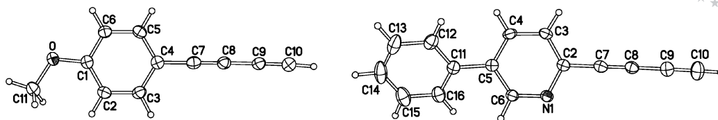
Figure 1. Molecular structures of 5c (left) and 10a (right) showing thermal ellipsoids at 50% probability level. Bond lengths [Å]: C(Ar)–C(7) 1.435(3) and 1.436(2), C(7)–C(8) 1.203(3) and 1.200(2), C(8)–C(9) 1.380(3) and 1.371(2), C(9)–C(10) 1.187(3) and 1.187(2), respectively. The angle between the aromatic ring planes in 10a is 32°.
