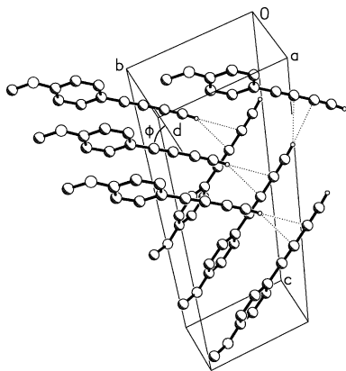
Figure 2. Crystal structure of 5c (H atoms, except acetylene ones, are omitted).
