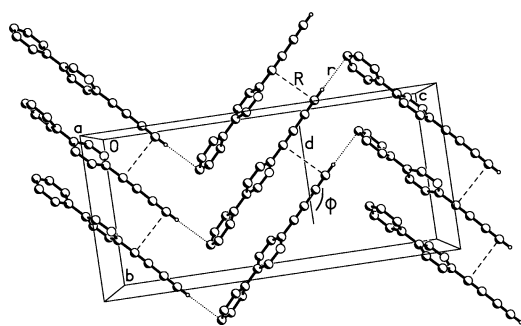
Figure 3. Crystal structure of 10a (H atoms, except acetylene ones, are omitted).
